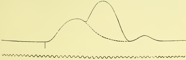
FIG. 13. TRACING OF A DOUBLE MUSCLE-CURVE.
